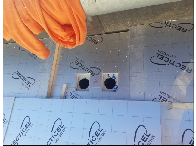
Installation of PIR Thermal insulation
