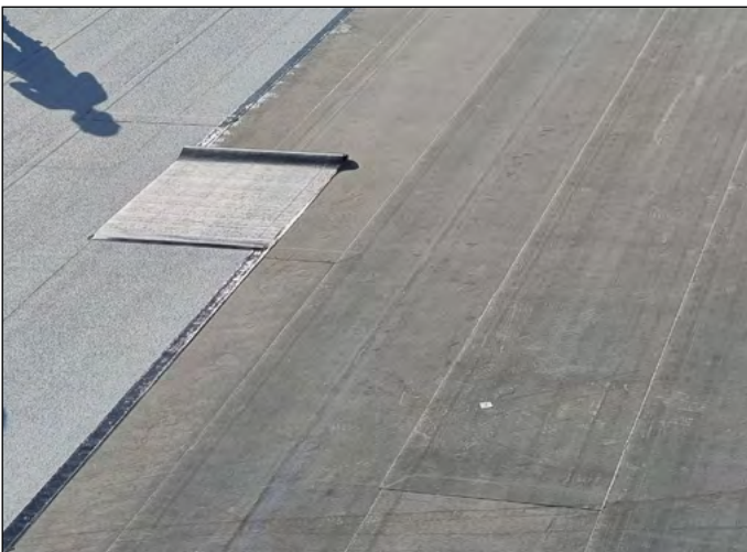
Base sheet installed, with cap sheet being application underway
