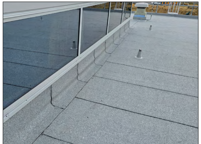
Detailing under window
