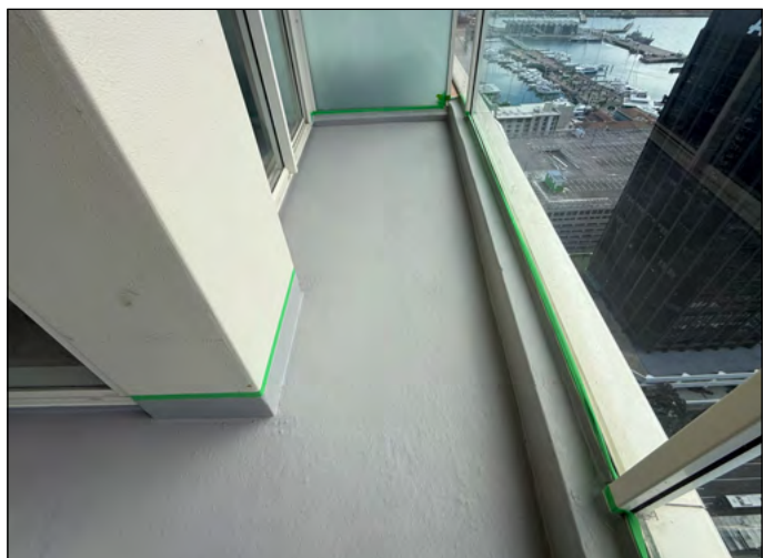
Application of Dextr with Traxx 2000 W/C as the topcoat
