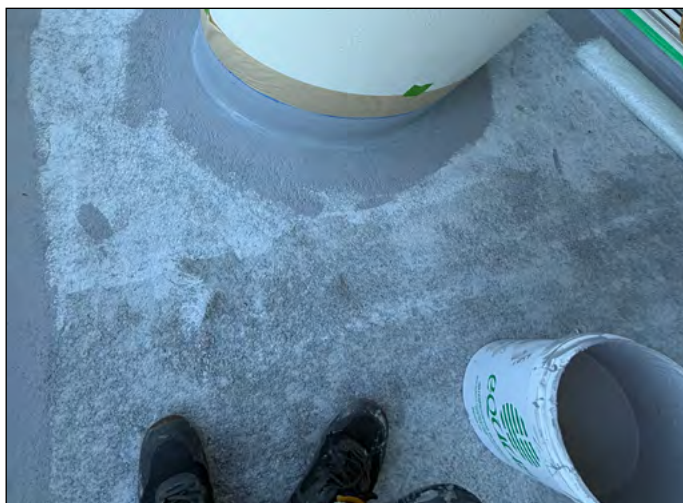
Application of the Chevaline Dextr system onto the concrete screed
