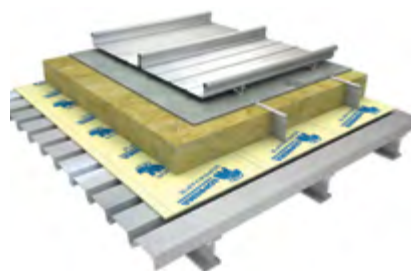
DOUBLE-SKIN METAL ROOF
