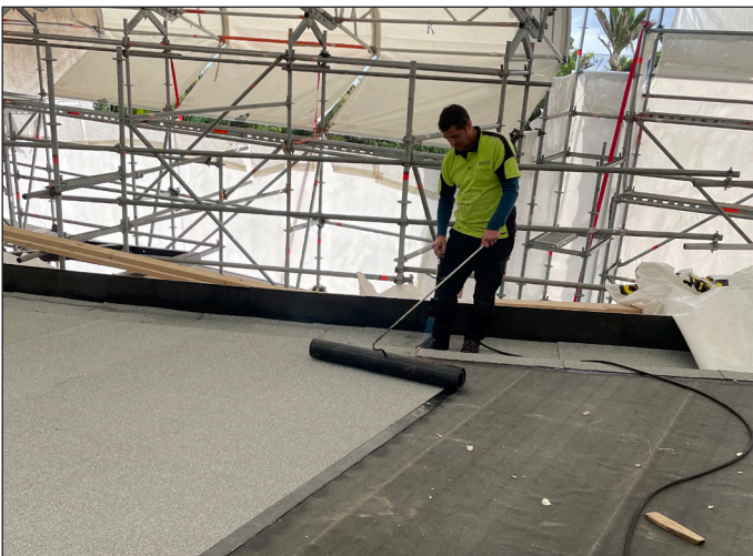
DUO LANDSCAPE cap sheet torched over base sheet
