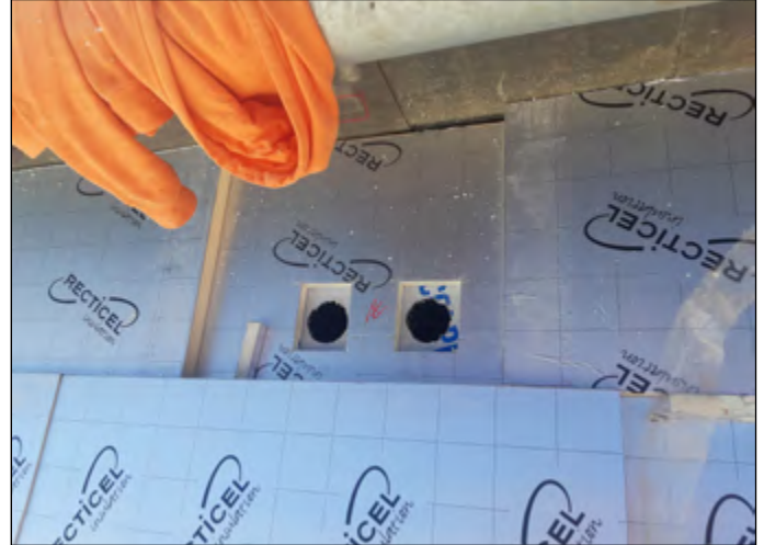
Installation of PIR thermal insulation
