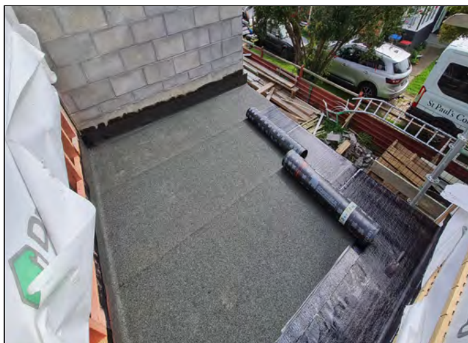
Dark grey cap sheet being applied
