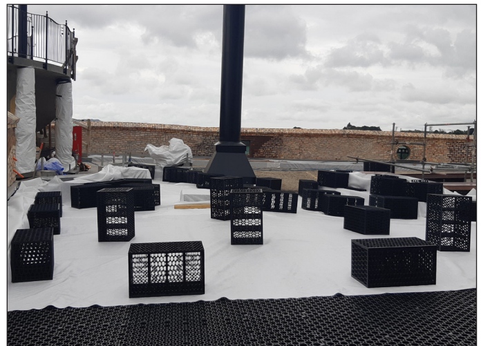
Drainage cell installation over DUO Landscape membrane before the green roof installation
