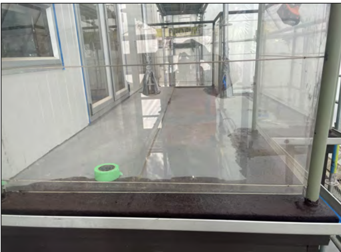
Application of second layer of EASY FLASHING
