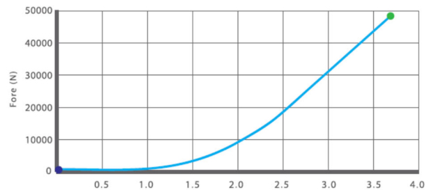
COMPRESSION TEST (COLD -40°)
