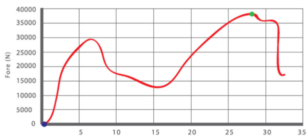
COMPRESSION TEST (HOT 23°)
