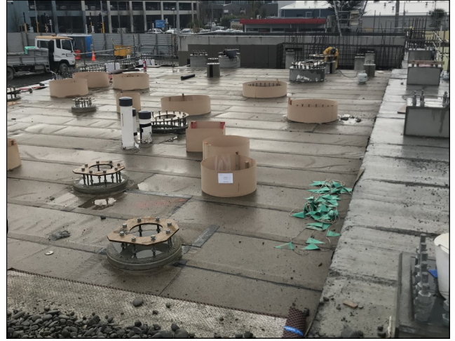
DeboFlex 3.5 Special detailing to piles
