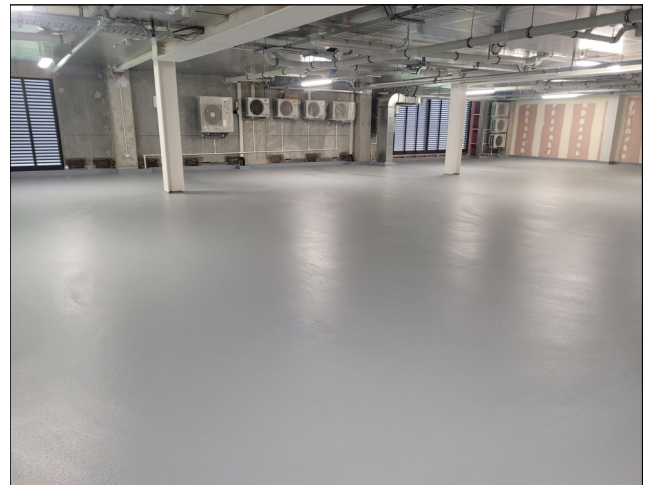
Topcoat of Matacryn applied
