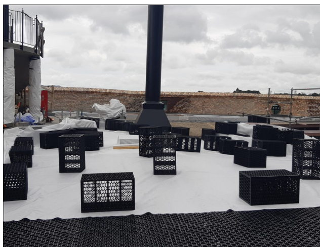
Drainage cell installation over Duo Landscape membrane before the green roof installation
